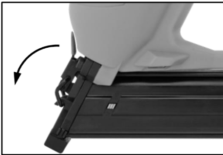
Fig. D – Removing a jammed nail
